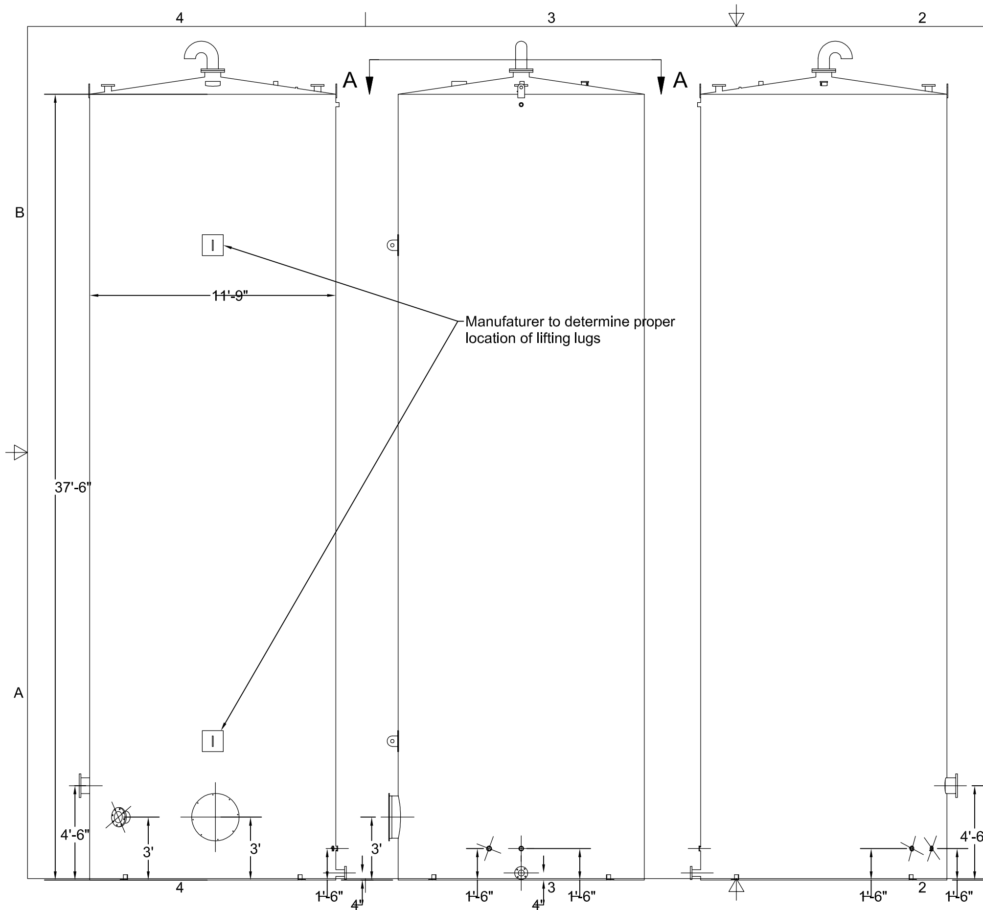
VIEW A-A SCALE 1 / 50
